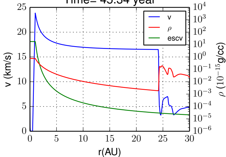
Time= 45.34 year
